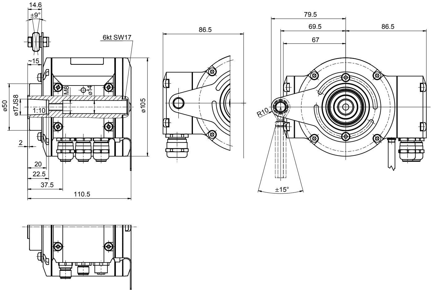
Cone shaft
