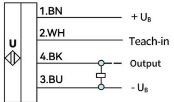
PNP
