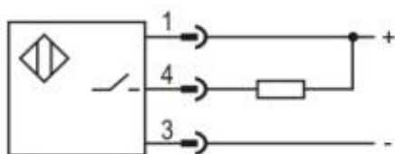
NPN NO
