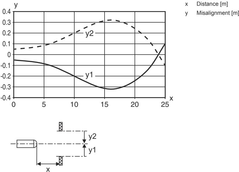
Typ. response behavior (TKS100x100)
