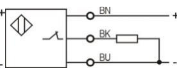
PNP NC
