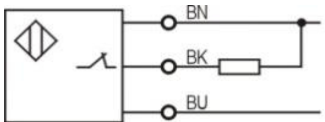
NPN NC
