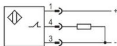
PNP NC
