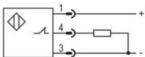
NPN NC
