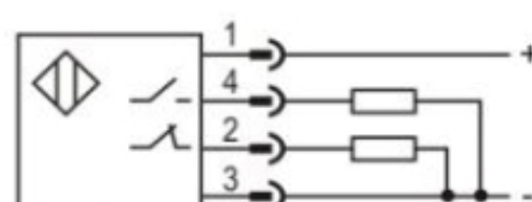
PNP NO+NC
