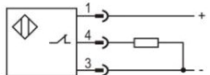
PNP NC
