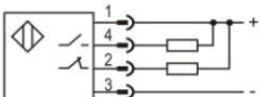
NPN NO+NC
