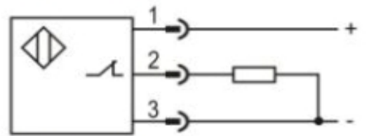
PNP NC
