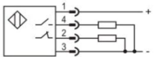
PNP NO+NC
