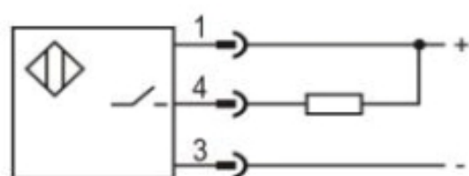
NPN NO
