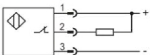
NPN NC
