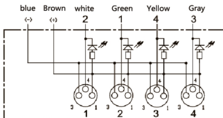
LED Indicator:NPN
