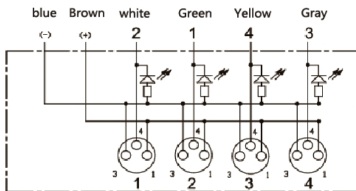
LED Indicator:PNP
