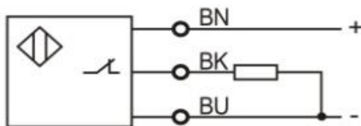
PNP NC
