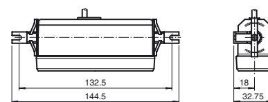
Mounting dimensions with mounting bracket set AIR30
