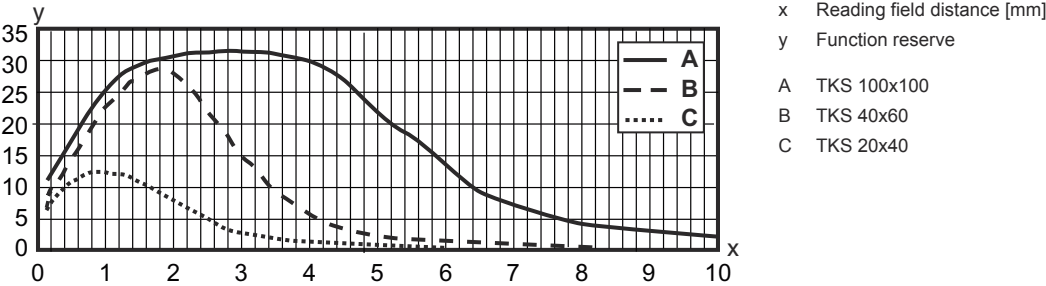
Typ. response behavior (TKS100x100)
