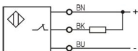
NPN NC
