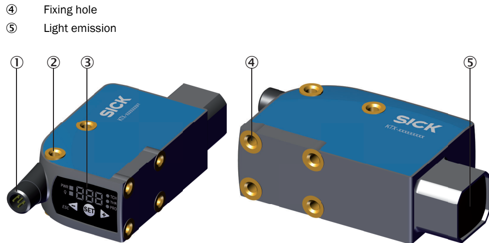
Figure 5: KTX Prime long sensing range light emission short housing side
