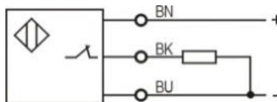
PNP NC
