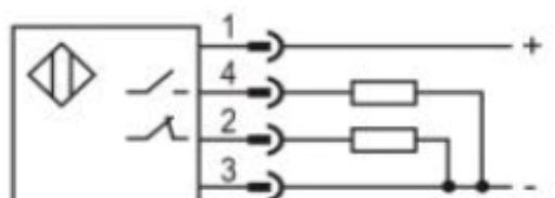
PNP NO+NC
