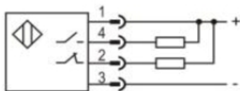
NPN NO+NC
