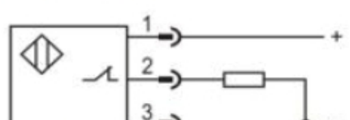
PNP NC
