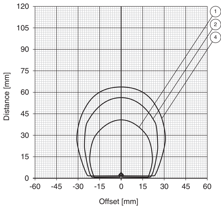
Reading range on steel IPC02-50..
