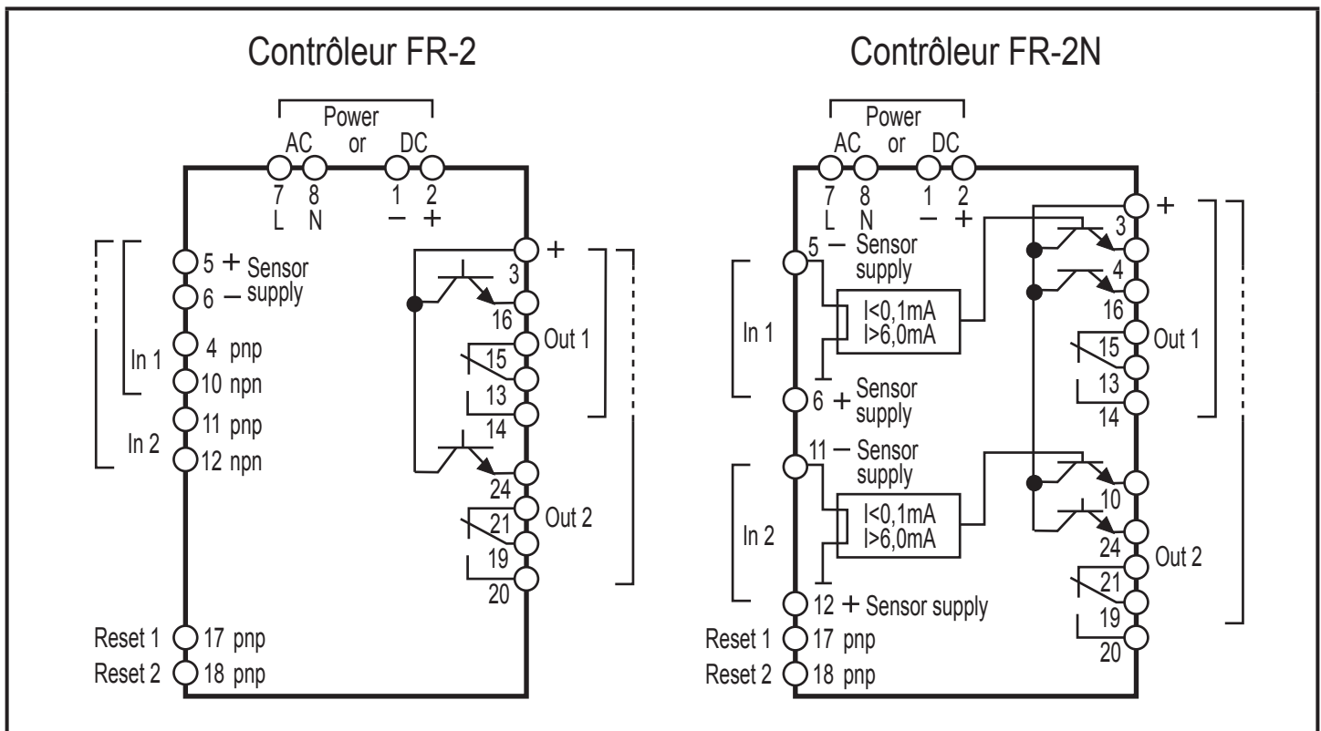
Raccordement des bornes
