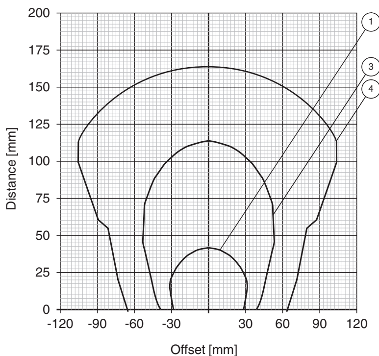
Reading range in air IQC22-C4
