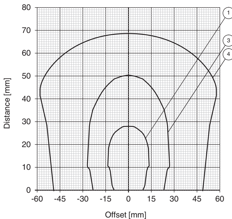
Reading range in air IQC33-30
