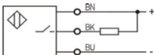
NPN NO
