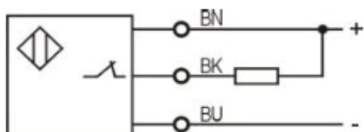
NPN NC
