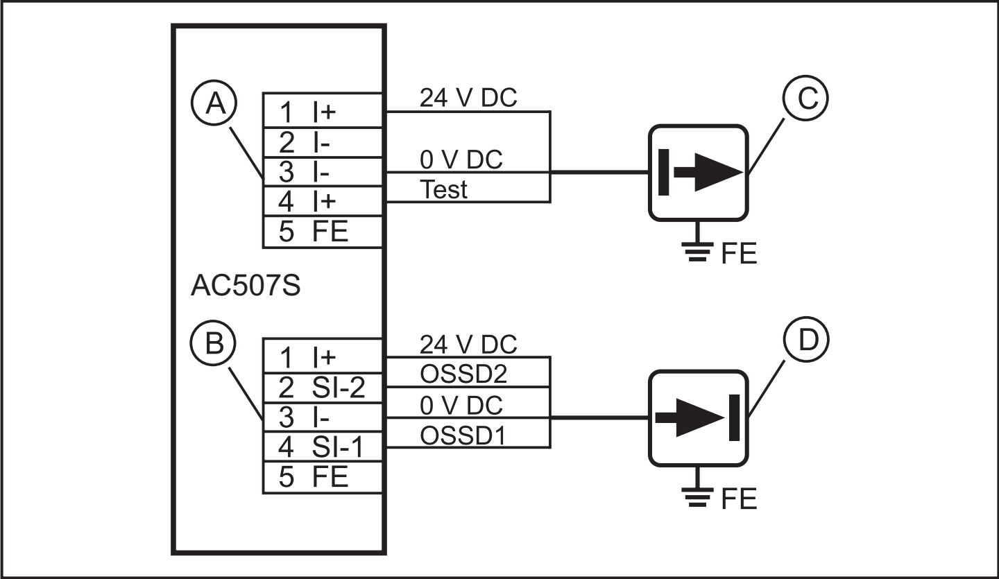
A: socket 3 / B: socket 1 / C: transmitter / D: receiver
