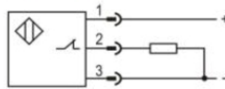
PNP NC
