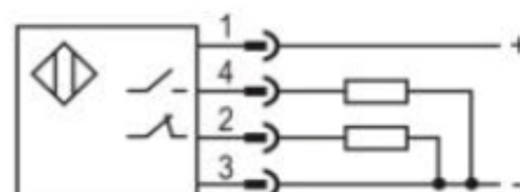
PNP NO+NC
