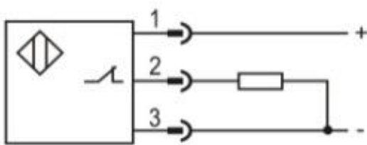
PNP NC
