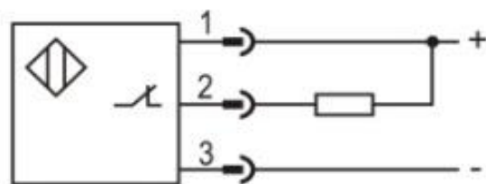
NPN NC
