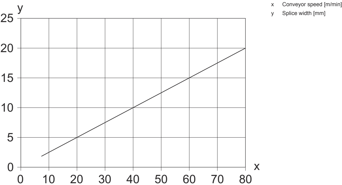
Splice width in dependence of web speed
