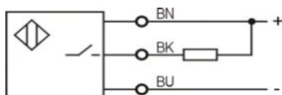
NPN NO
