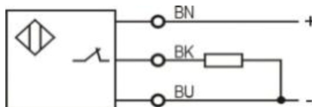
PNP NC
