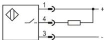
NPN NO
