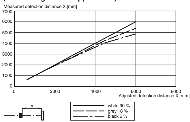
Difference in detection distance (with background suppression)
