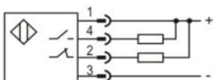
NPN NO+NC
