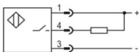
NPN NO
