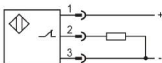
PNP NC
