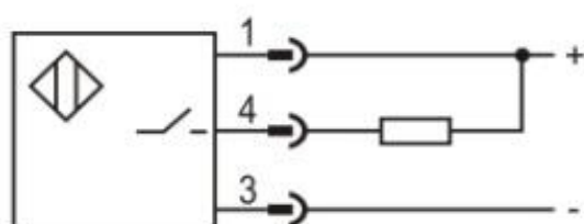
NPN NO
