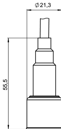
Housing with cable outlet, 3-wire
