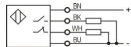
PNP NO+NC
