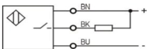
NPN NO
