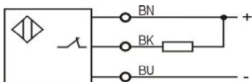
NPN NC
