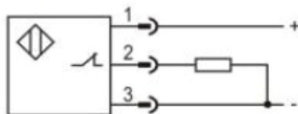
PNP NC
