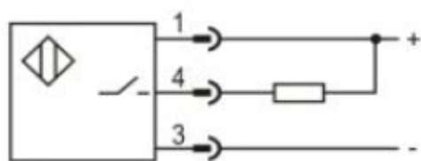
NPN NO
