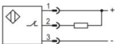
NPN NC
