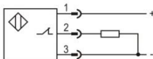
PNP NC
