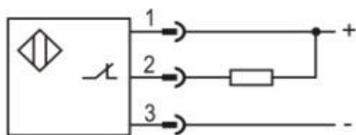
NPN NC
