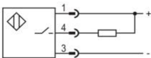
NPN NO
