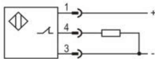
PNP NC
