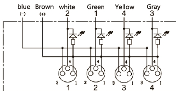
LED Indicator:NPN
