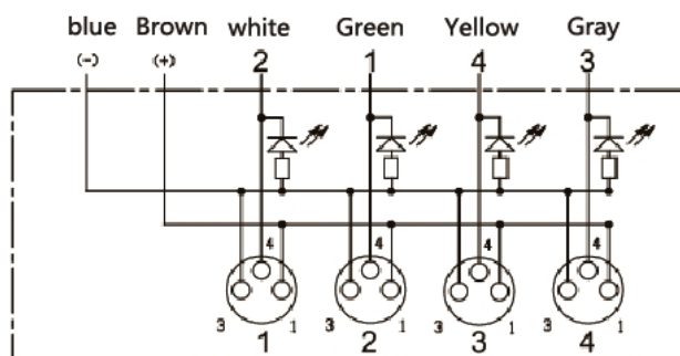
LED Indicator:PNP
