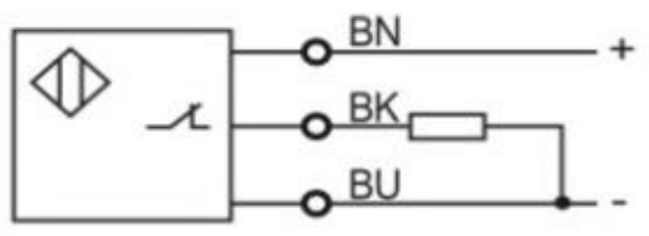
PNP NC
