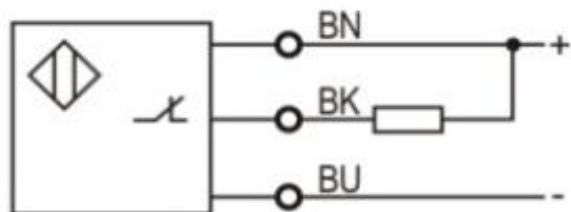
NPN NC
