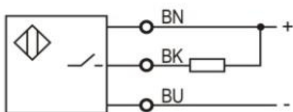
NPN NO
