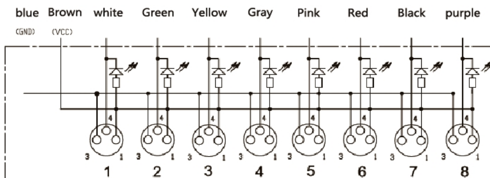
LED Indicator:NPN
