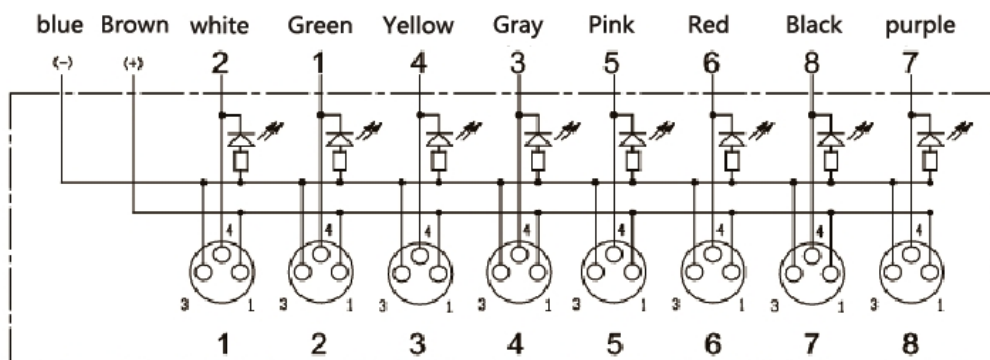
LED Indicator:PNP
